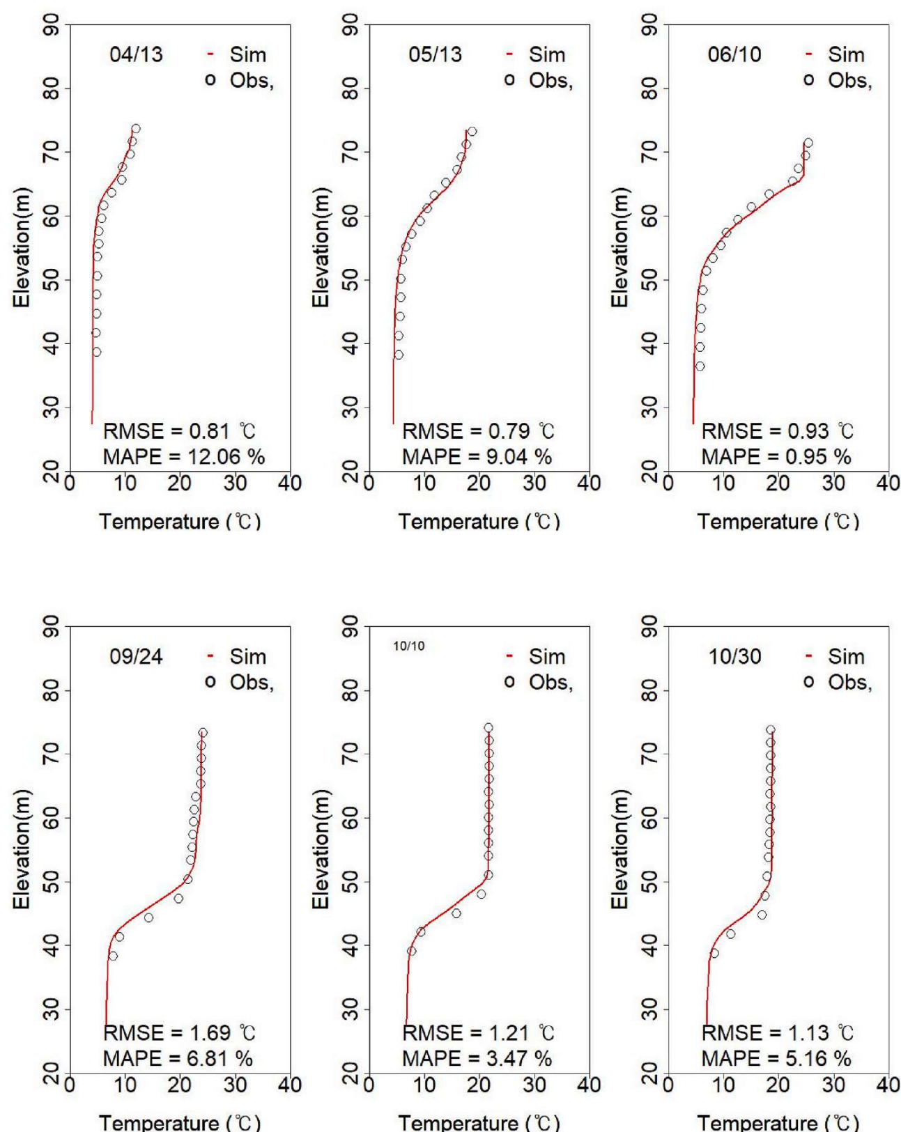
Fig. 2. Comparison of the observed and simulated water temperature profiles at the DC2 station.
